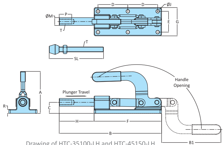
Drawing of HTC-35100-LH and HTC-45150-LH
